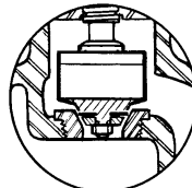
DUAL-SEAL WAFER DISC AND RENEWABLE SEAT
