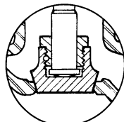
PLUG TYPE DISC
